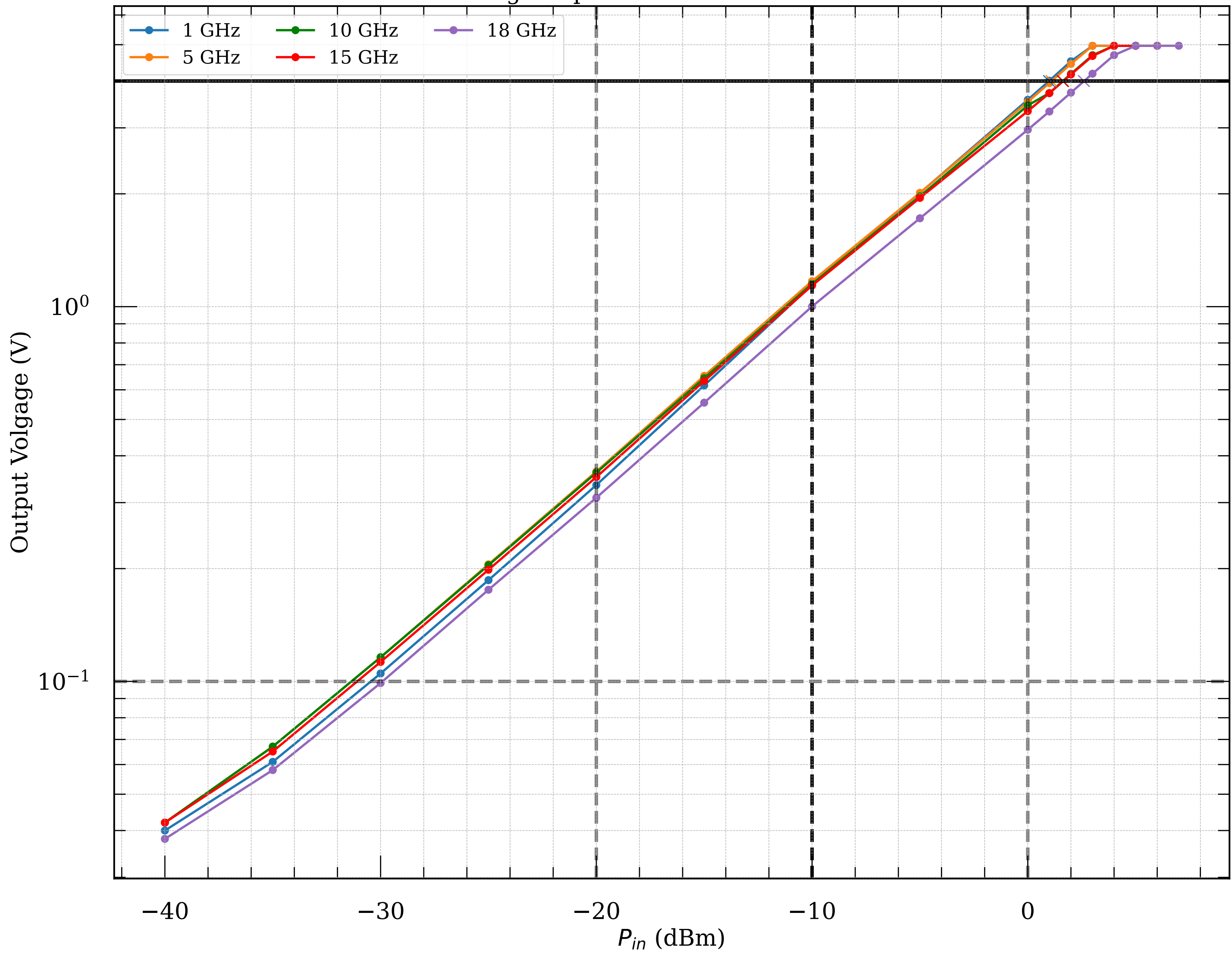
Measured voltage-to-power curve of detector module065v2
